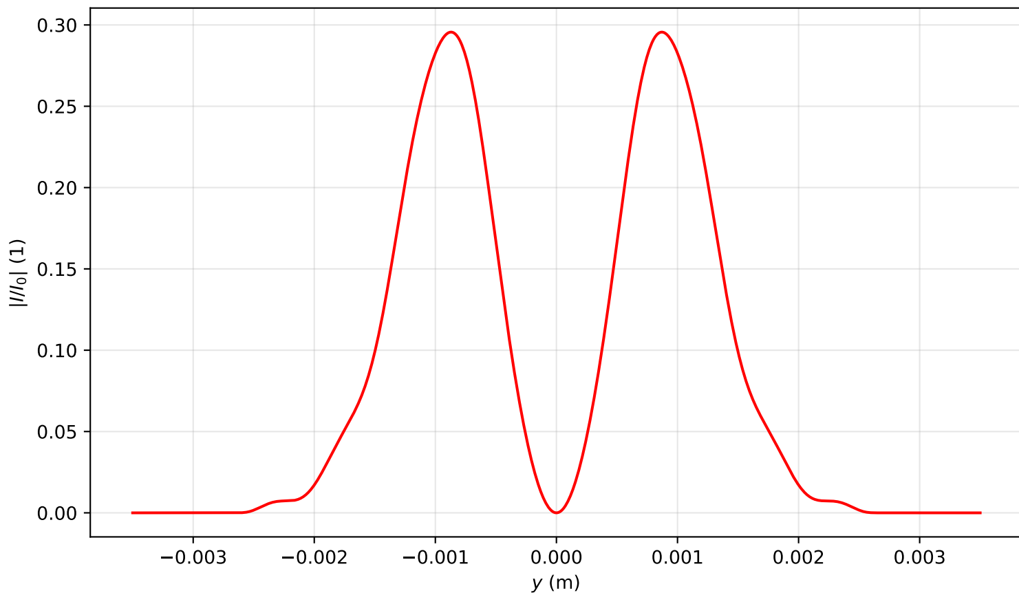
Intensity profile I(x=0, y, z=3.423)/I_0 , P_{in}=2.0P_{cr} , artificial time
